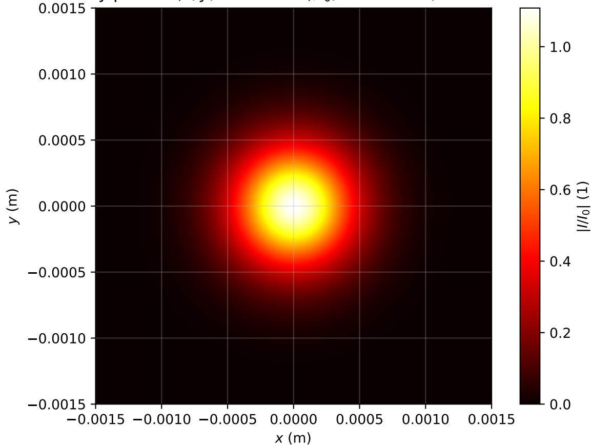
Intensity profile I(x, y, z = 0.557m)/I_0 , P_{in}=0.7P_{cr} , artificial time
